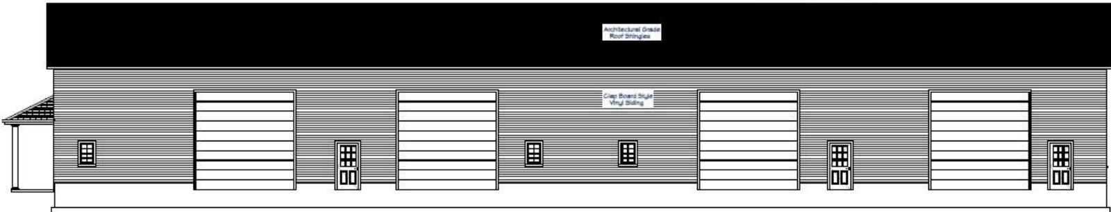
FRONT ELEVATION
